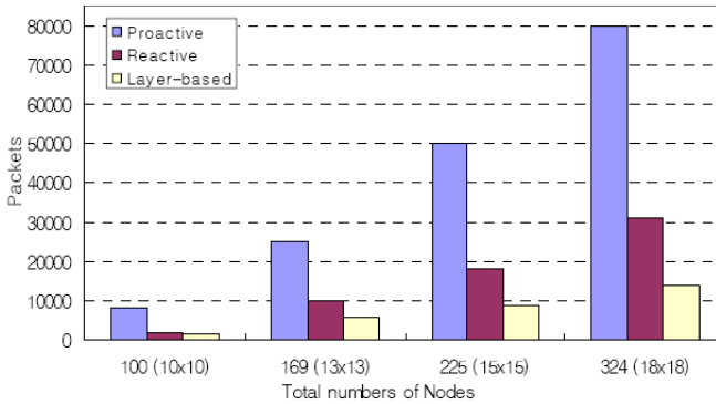
Fig. 4. Communication Overhead
