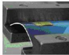
Fig. 19. Disconnection between COB and Antenna (after 2,500 times stressed)
