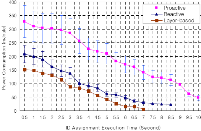
Fig. 5. Energy Consumption
