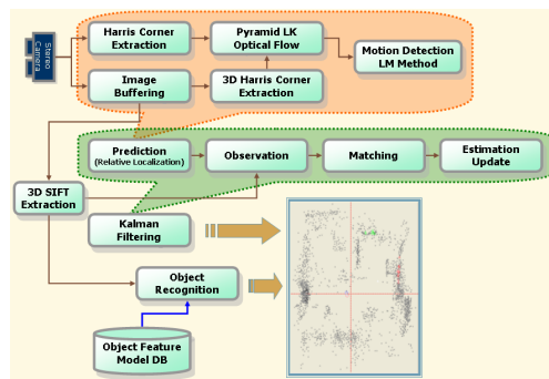
Fig. 1. Block diagram of the proposed map-building
