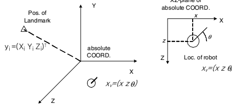
Fig. 2. System coordinate for the robot location and the landmark position
