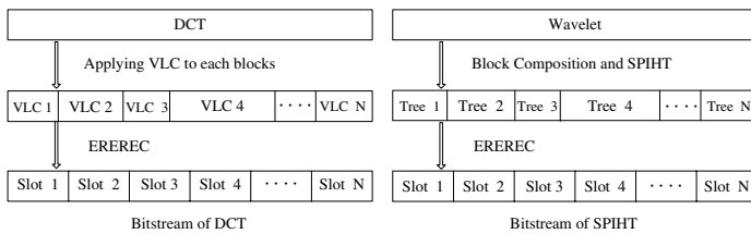
Fig. 3. Bit-Streaming of SPIHT and DCT based coding for EREREC
