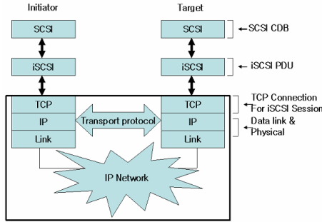
Fig. 1. iSCSI (Internet Small Computer System Interface) Protocol Architecture
