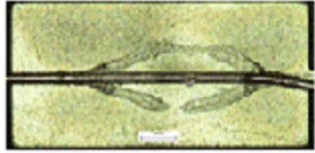
Fig. 11. Direct bonding between □ shaped antenna ends and electrodes of COB module Fig. 12. Microscopic view of bonded antenna
