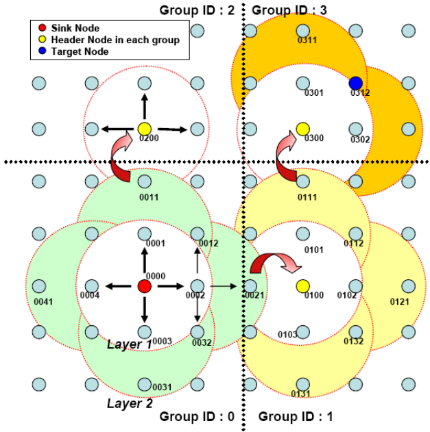
Fig. 3. ID Assignment in Children Grouping Algorithm
