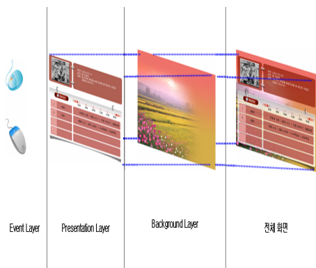
Fig. 2. A compunction screen composes a rendering engine
