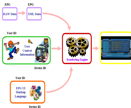
Fig. 3. Three EPG output structure charts which used different context information
