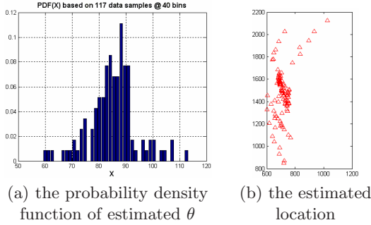
Fig. 3. The statistics of the robot localization
