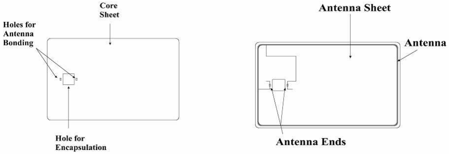
Fig. 9. A core sheet and an antenna sheet for an inlay sheet used in the proposed method
