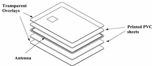
Fig. 1. Laminating sheets for a card body
