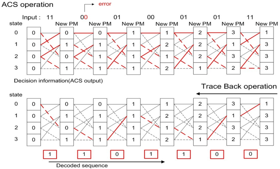
Fig. 1. The operation of the TB algorithm
